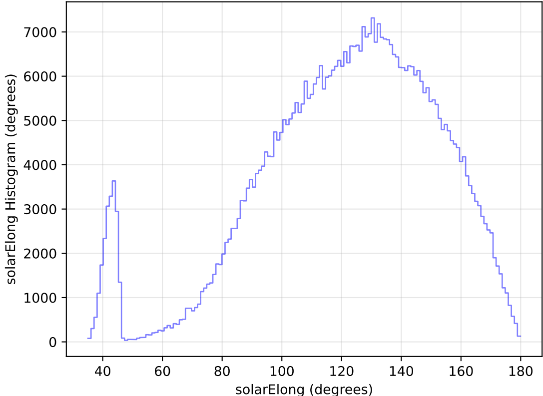
too_elab_heavy_r64_d2_ugrizy_v3.4_10yrs All sky i band: solarElong Histogram
