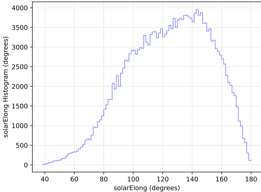
too_elab_heavy_r64_d2_ugrizy_v3.4_10yrs All sky g band: solarElong Histogram
