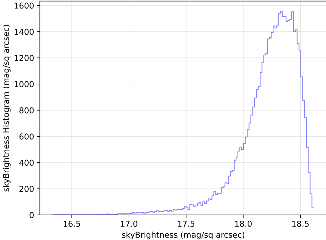
too_elab_heavy_r64_d2_ugrizy_v3.4_10yrs Yr 1 y band: skyBrightness Histogram
