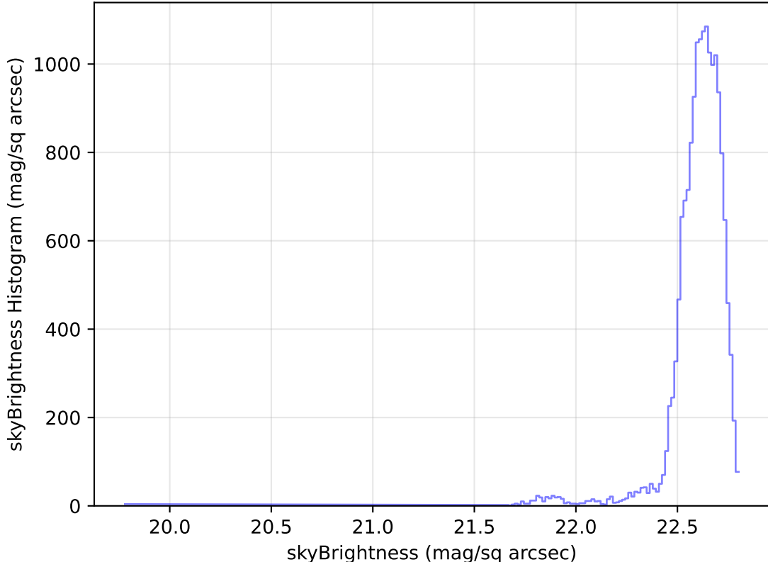
too_elab_heavy_r64_d2_ugrizy_v3.4_10yrs Yr 1 u band: skyBrightness Histogram
