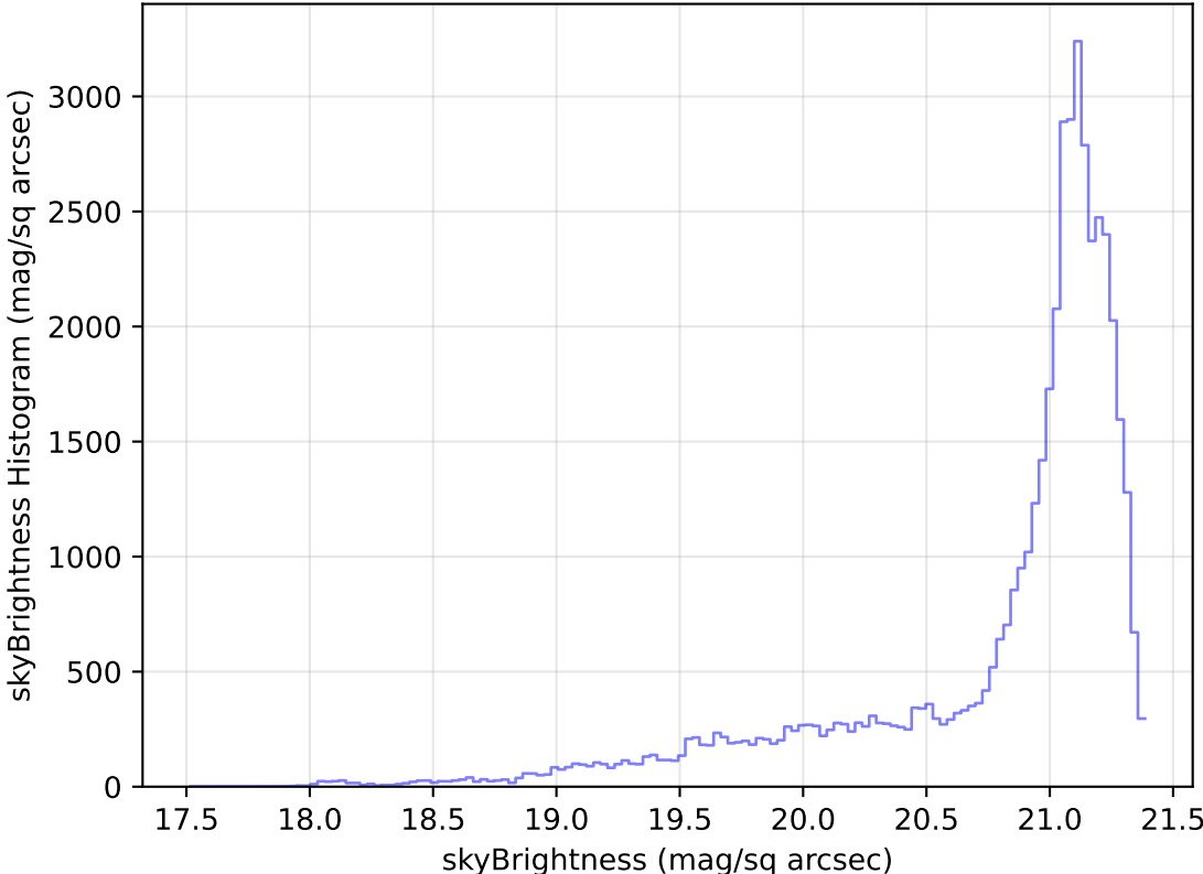
too_elab_heavy_r64_d2_ugrizy_v3.4_10yrs Yr 1 r band: skyBrightness Histogram
