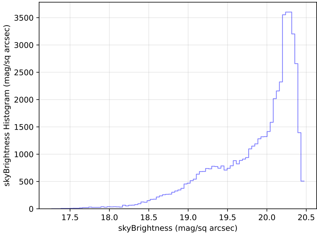
too_elab_heavy_r64_d2_ugrizy_v3.4_10yrs Yr 1 i band: skyBrightness Histogram
