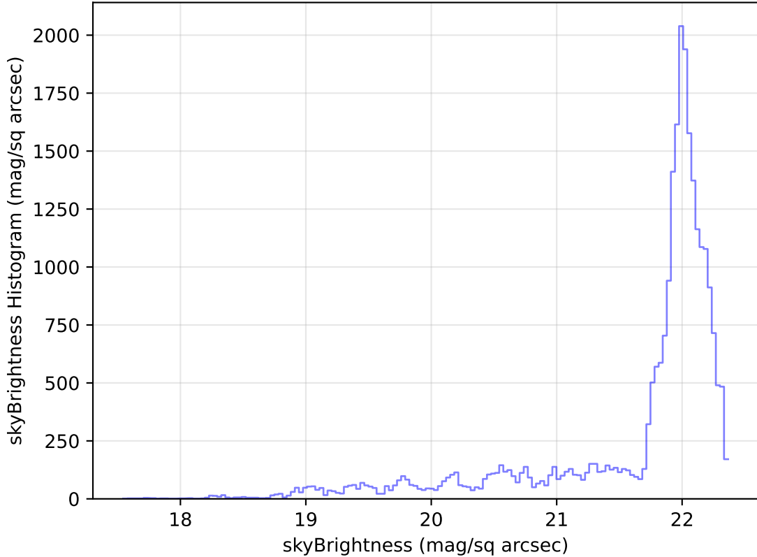
too_elab_heavy_r64_d2_ugrizy_v3.4_10yrs Yr 1 g band: skyBrightness Histogram
