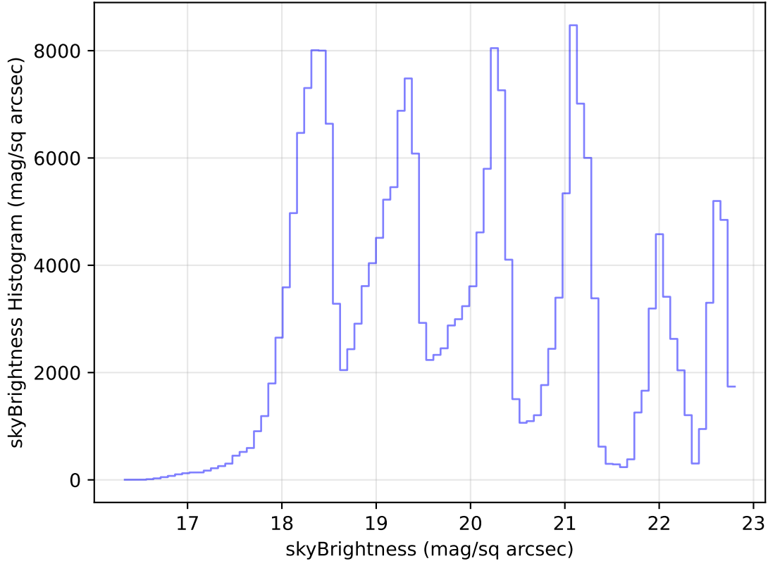
too_elab_heavy_r64_d2_ugrizy_v3.4_10yrs Yr 1 all bands: skyBrightness Histogram
