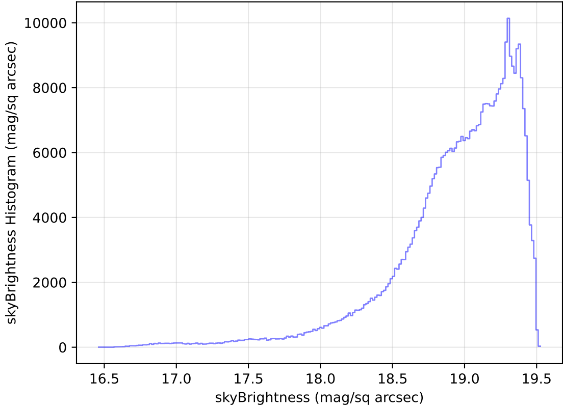
too_elab_heavy_r64_d2_ugrizy_v3.4_10yrs WFD z band: skyBrightness Histogram
