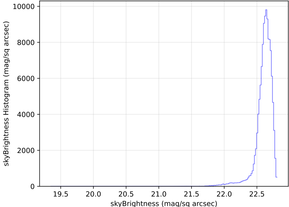
too_elab_heavy_r64_d2_ugrizy_v3.4_10yrs WFD u band: skyBrightness Histogram
