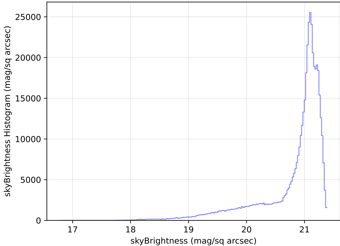
too_elab_heavy_r64_d2_ugrizy_v3.4_10yrs_WFD_r_band: skyBrightness Histogram
