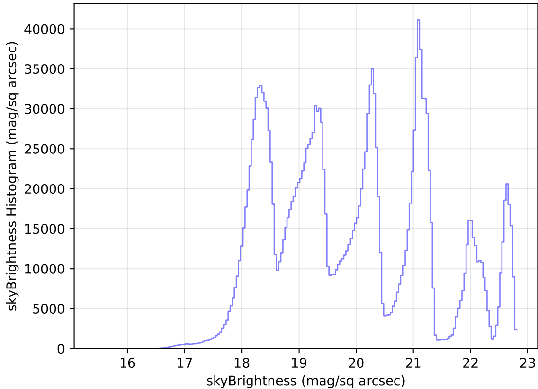
too_elab_heavy_r64_d2_ugrizy_v3.4_10yrs WFD all bands: skyBrightness Histogram
