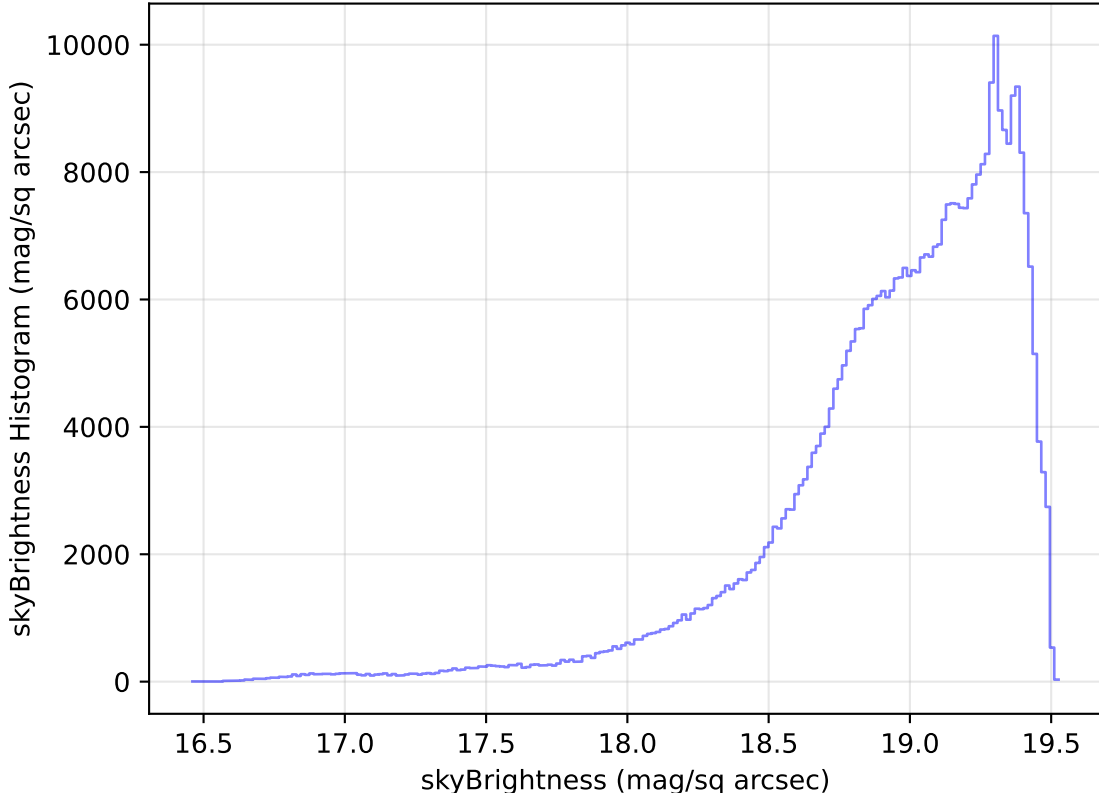
too_elab_heavy_r64_d2_ugrizy_v3.4_10yrs All sky z band: skyBrightness Histogram
