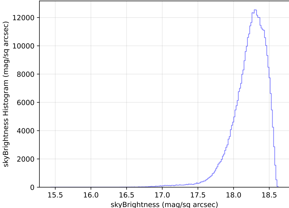
too_elab_heavy_r64_d2_ugrizy_v3.4_10yrs All sky y band: skyBrightness Histogram
