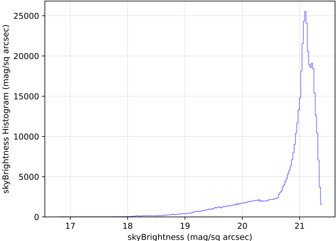
too_elab_heavy_r64_d2_ugrizy_v3.4_10yrs All sky r band: skyBrightness Histogram
