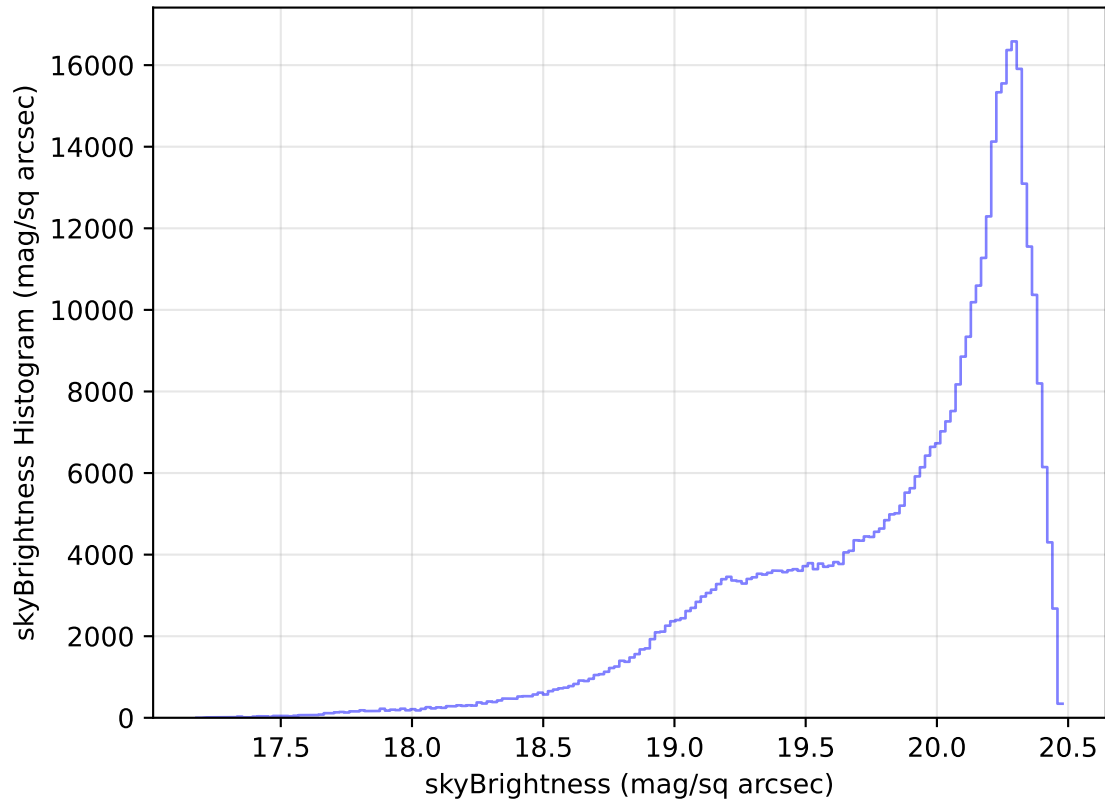
too_elab_heavy_r64_d2_ugrizy_v3.4_10yrs All sky i band: skyBrightness Histogram
