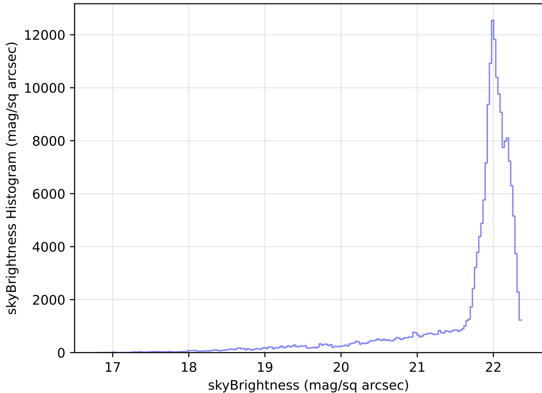
too_elab_heavy_r64_d2_ugrizy_v3.4_10yrs All sky g band: skyBrightness Histogram
