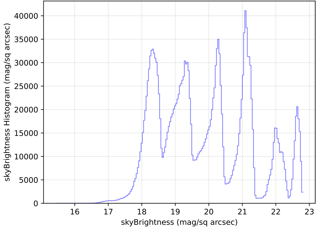
too_elab_heavy_r64_d2_ugrizy_v3.4_10yrs All sky all bands: skyBrightness Histogram
