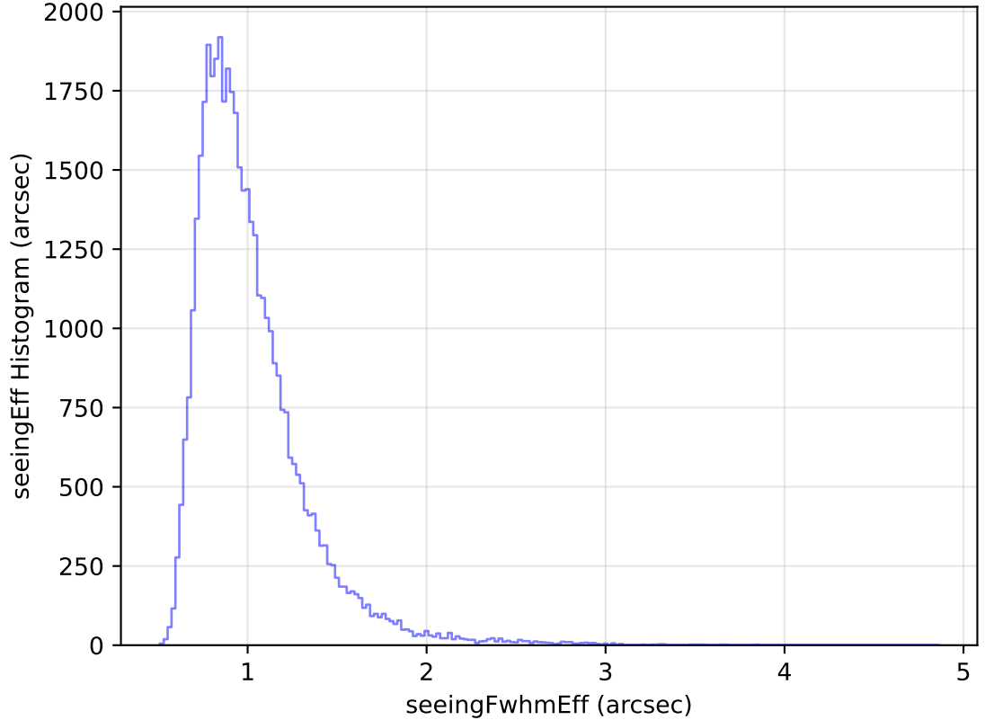
too_elab_heavy_r64_d2_ugrizy_v3.4_10yrs Yr 1 z band: seeingEff Histogram
