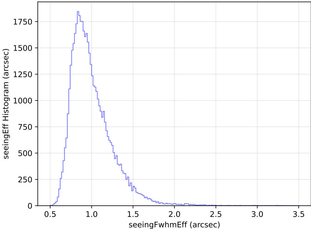
too_elab_heavy_r64_d2_ugrizy_v3.4_10yrs Yr 1 y band: seeingEff Histogram
