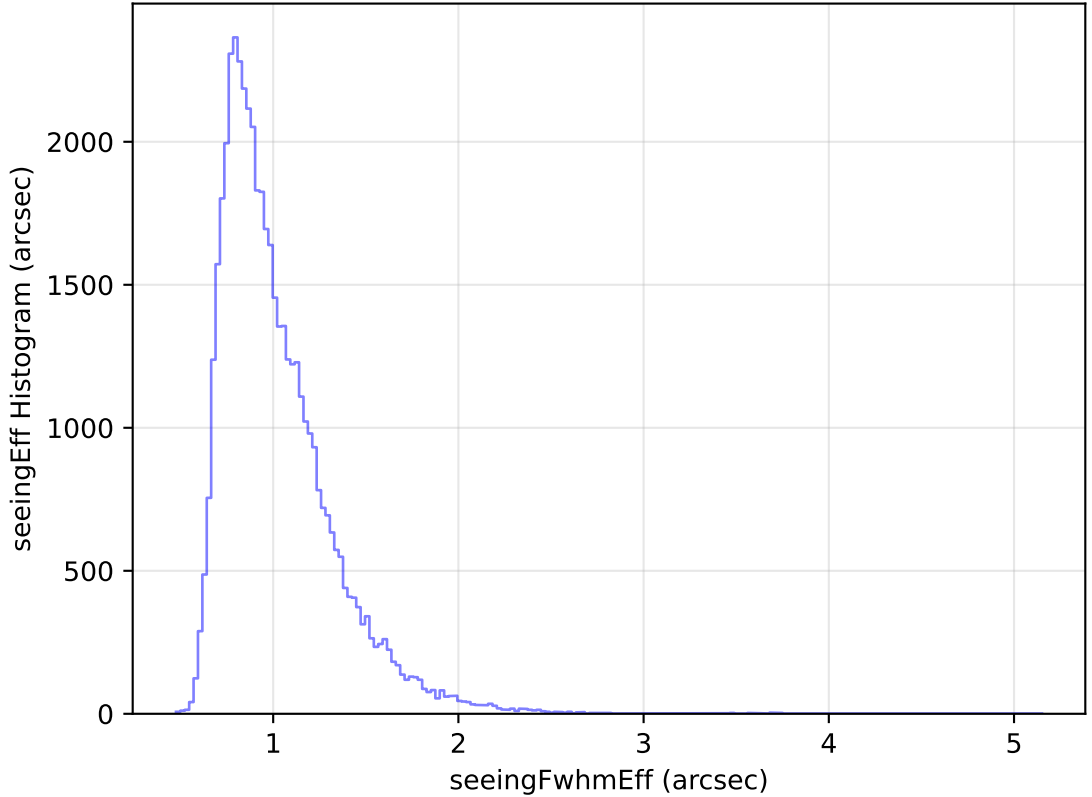
too_elab_heavy_r64_d2_ugrizy_v3.4_10yrs Yr 1 r band: seeingEff Histogram
