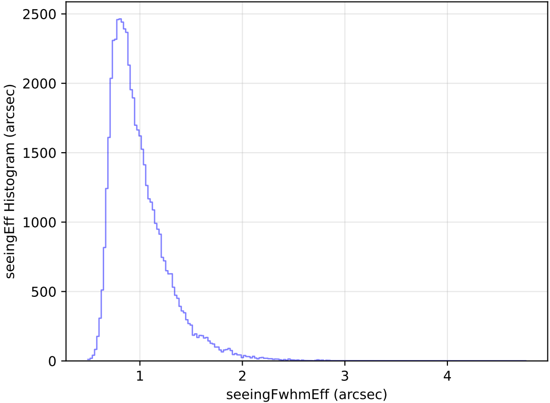
too_elab_heavy_r64_d2_ugrizy_v3.4_10yrs Yr 1 i band: seeingEff Histogram
