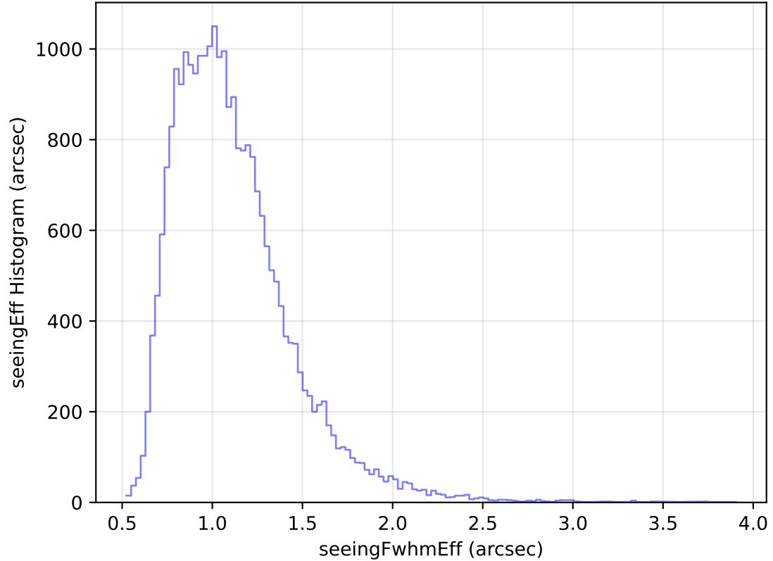
too_elab_heavy_r64_d2_ugrizy_v3.4_10yrs Yr 1 g band: seeingEff Histogram
