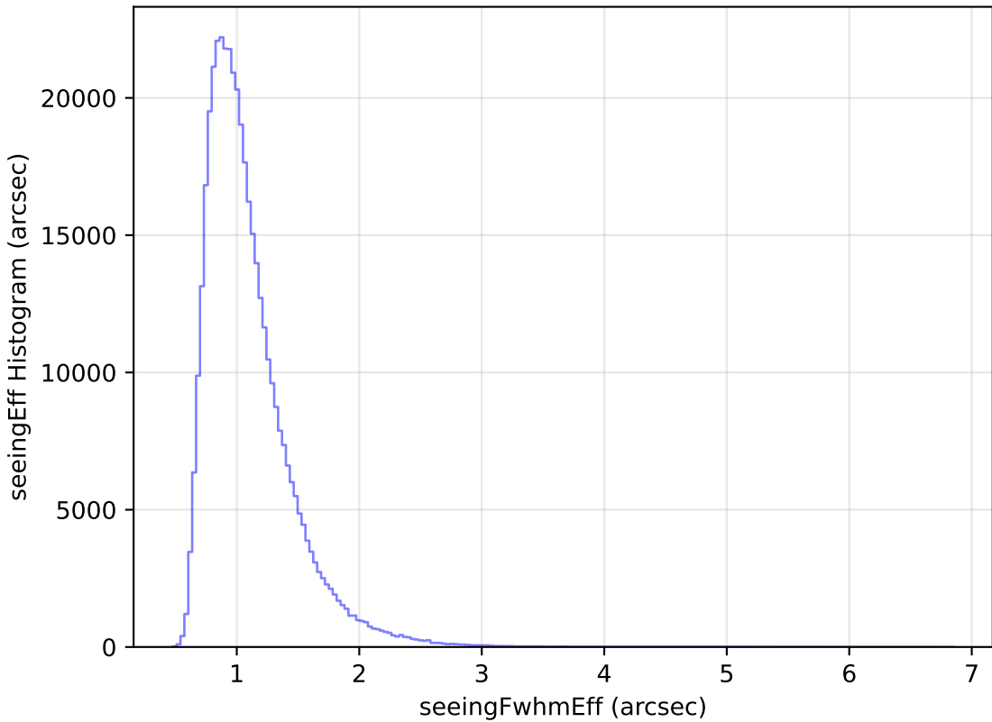
too_elab_heavy_r64_d2_ugrizy_v3.4_10yrs WFD z band: seeingEff Histogram
