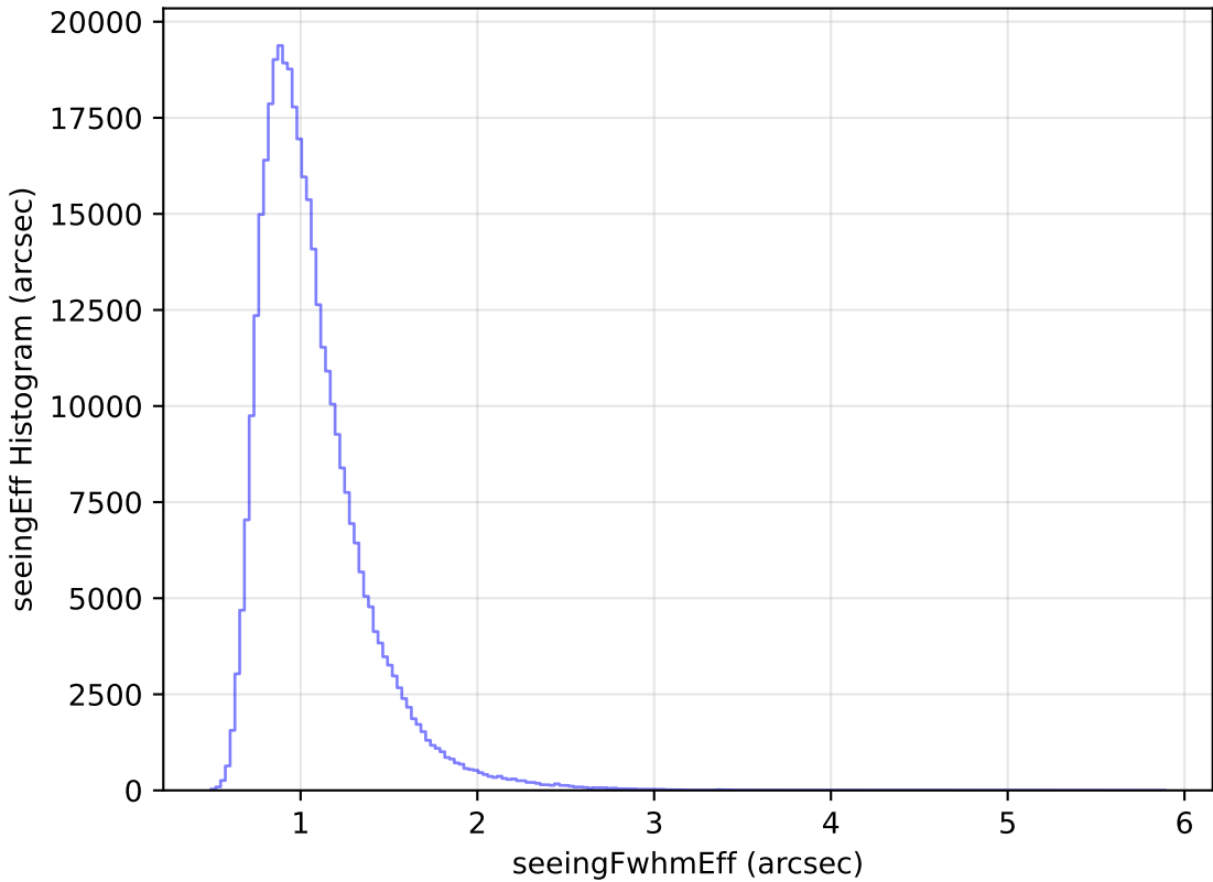
too_elab_heavy_r64_d2_ugrizy_v3.4_10yrs WFD y band: seeingEff Histogram
