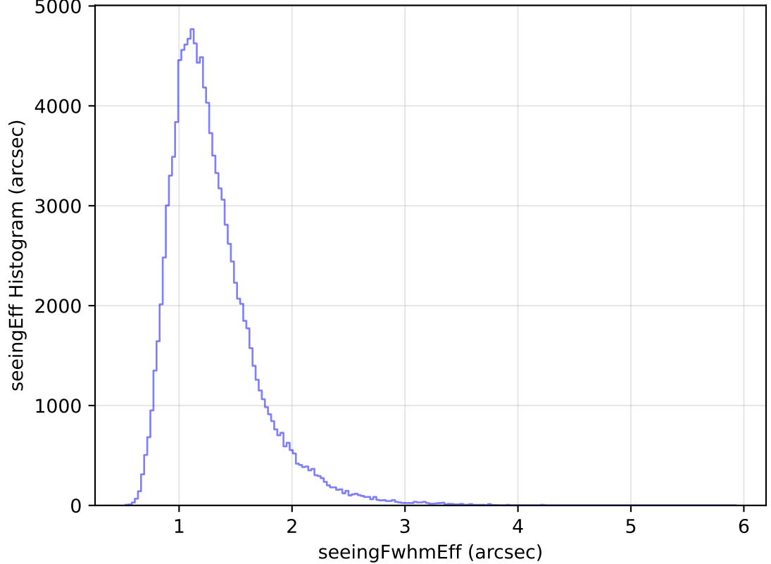
too_elab_heavy_r64_d2_ugrizy_v3.4_10yrs WFD u band: seeingEff Histogram
