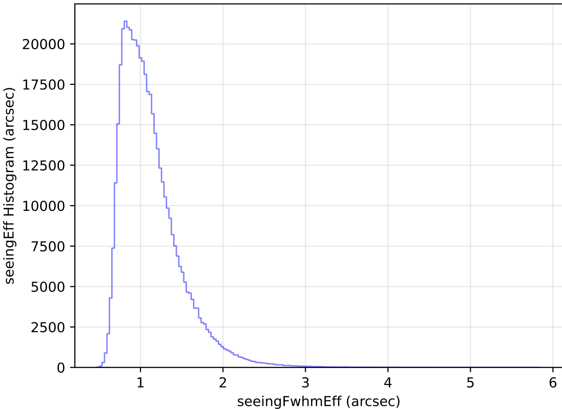
too_elab_heavy_r64_d2_ugrizy_v3.4_10yrs WFD r band: seeingEff Histogram
