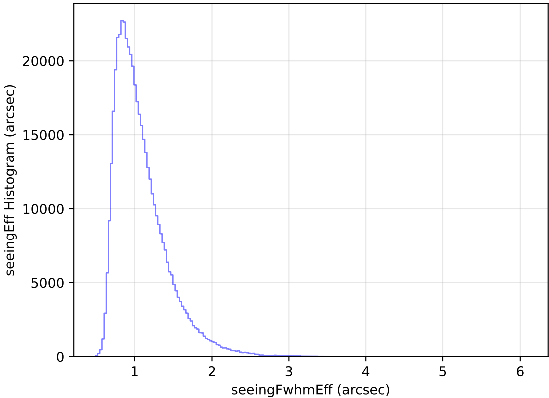
too_elab_heavy_r64_d2_ugrizy_v3.4_10yrs WFD i band: seeingEff Histogram
