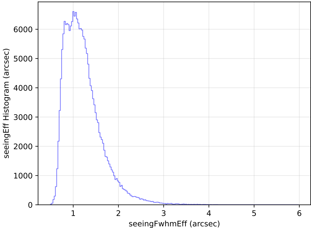
too_elab_heavy_r64_d2_ugrizy_v3.4_10yrs WFD g band: seeingEff Histogram
