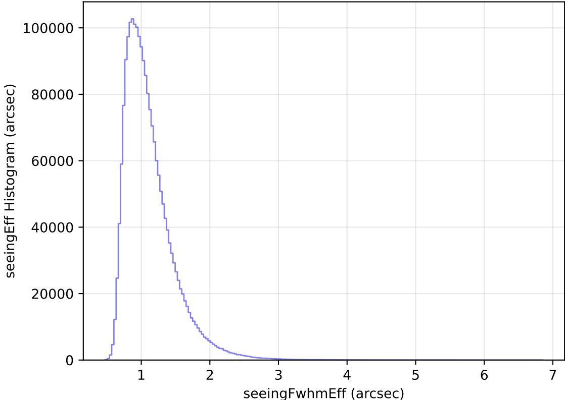
too_elab_heavy_r64_d2_ugrizy_v3.4_10yrs WFD all bands: seeingEff Histogram
