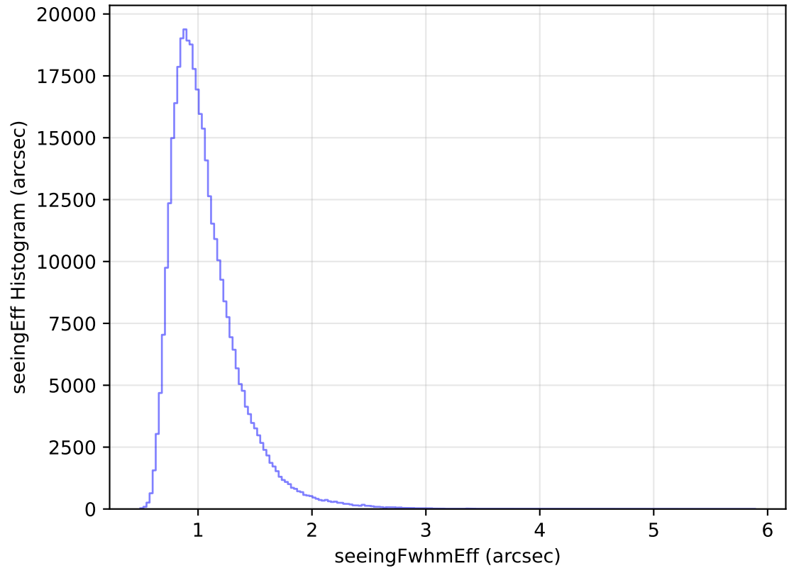
too_elab_heavy_r64_d2_ugrizy_v3.4_10yrs All sky y band: seeingEff Histogram
