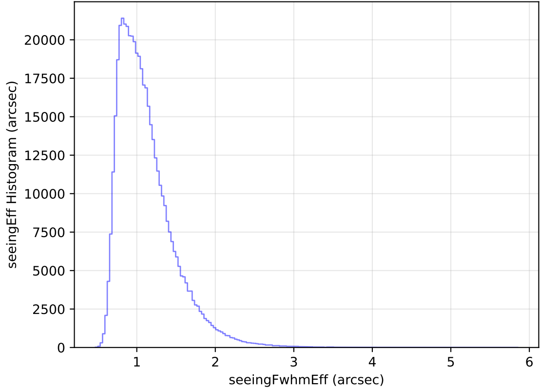
too_elab_heavy_r64_d2_ugrizy_v3.4_10yrs All sky r band: seeingEff Histogram
