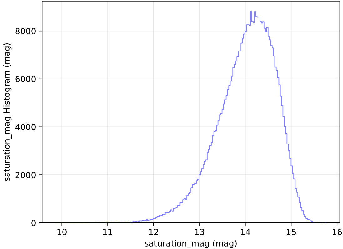
too_elab_heavy_r64_d2_ugrizy_v3.4_10yrs WFD z band: saturation_mag Histogram
