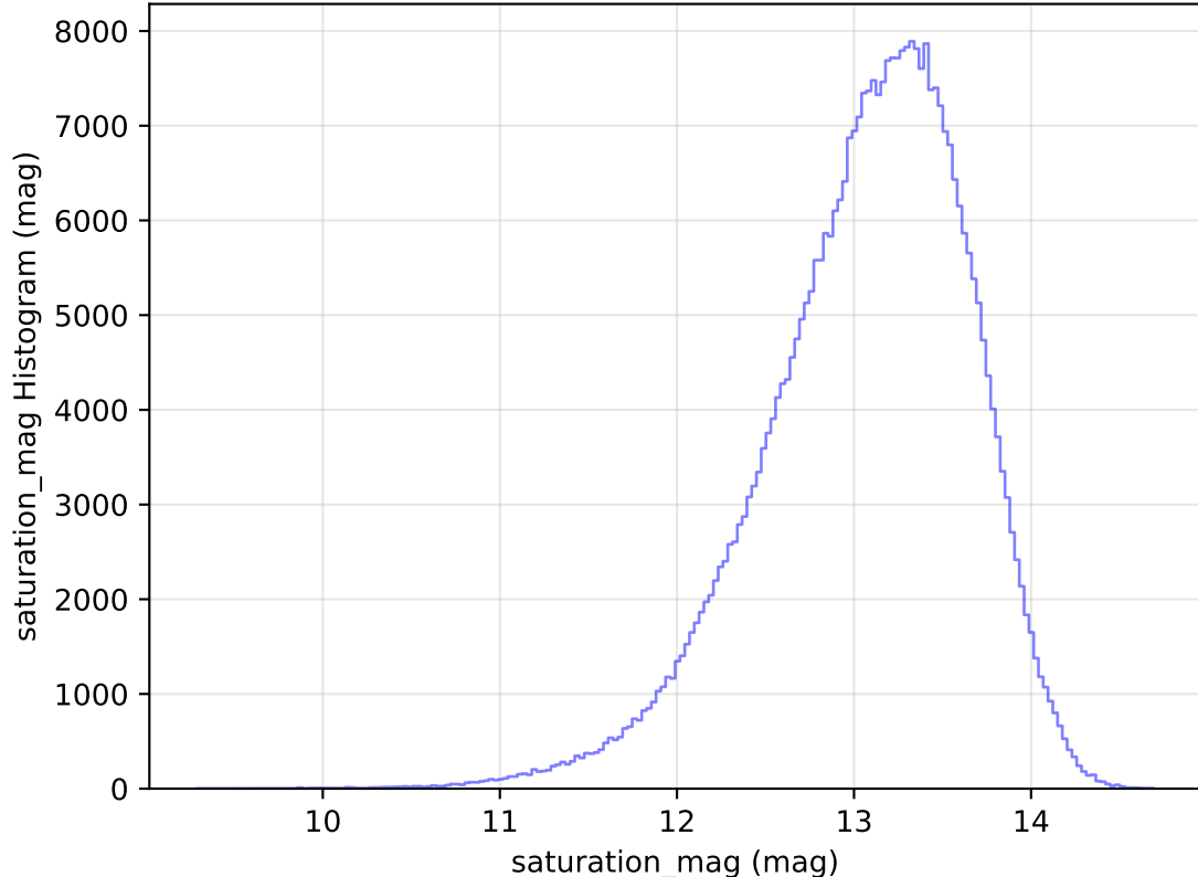
too_elab_heavy_r64_d2_ugrizy_v3.4_10yrs WFD y band: saturation_mag Histogram
