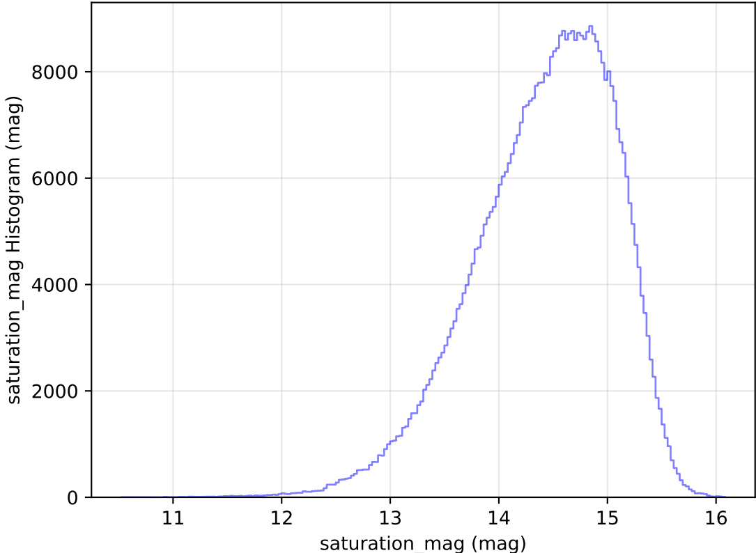
too_elab_heavy_r64_d2_ugrizy_v3.4_10yrs WFD i band: saturation_mag Histogram
