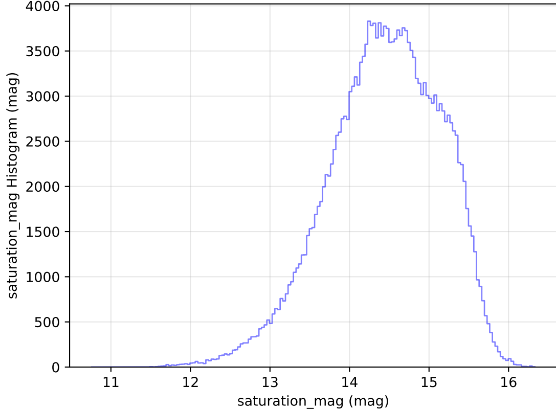
too_elab_heavy_r64_d2_ugrizy_v3.4_10yrs WFD g band: saturation_mag Histogram
