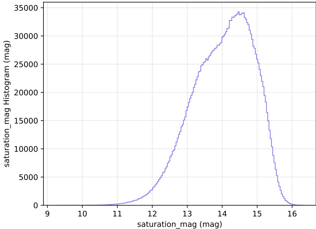
too_elab_heavy_r64_d2_ugrizy_v3.4_10yrs WFD all bands: saturation_mag Histogram
