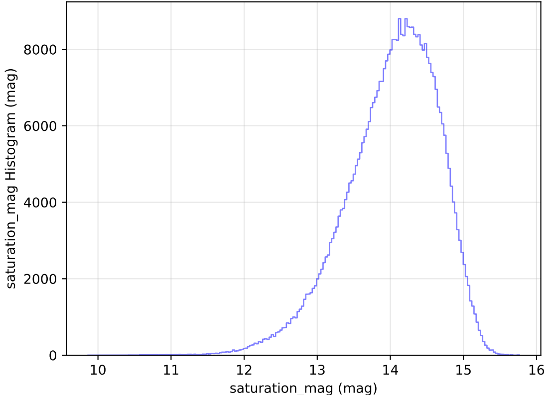
too_elab_heavy_r64_d2_ugrizy_v3.4_10yrs All sky z band: saturation_mag Histogram
