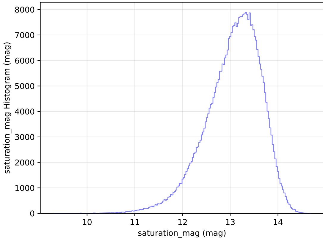
too_elab_heavy_r64_d2_ugrizy_v3.4_10yrs All sky y band: saturation_mag Histogram
