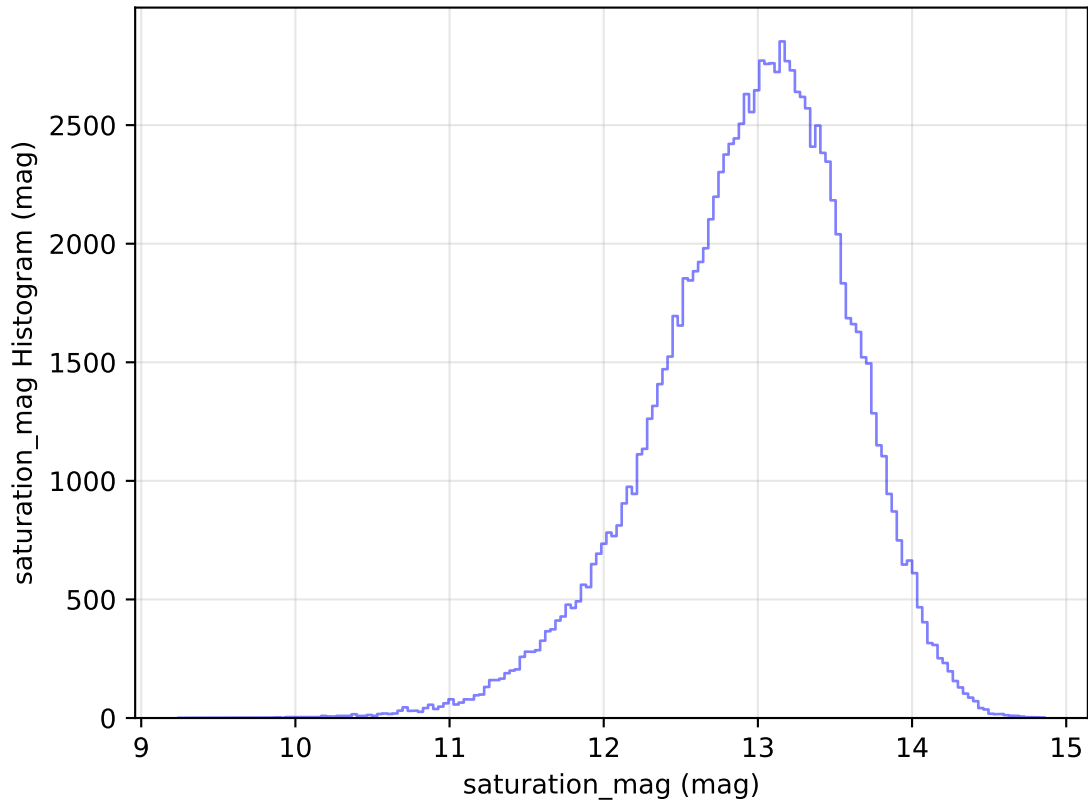
too_elab_heavy_r64_d2_ugrizy_v3.4_10yrs All sky u band: saturation_mag Histogram
