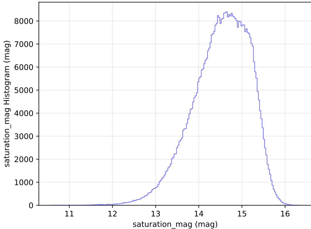
too_elab_heavy_r64_d2_ugrizy_v3.4_10yrs All sky r band: saturation_mag Histogram
