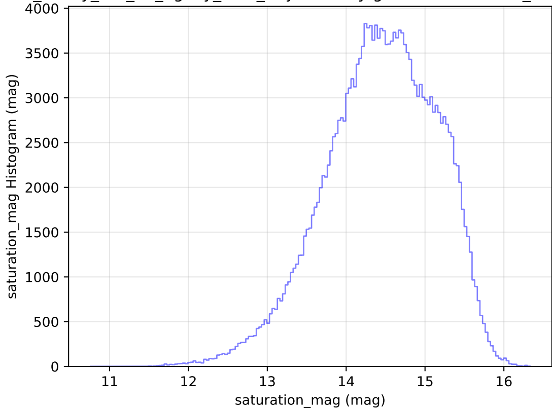
too_elab_heavy_r64_d2_ugrizy_v3.4_10yrs All sky g band: saturation_mag Histogram
