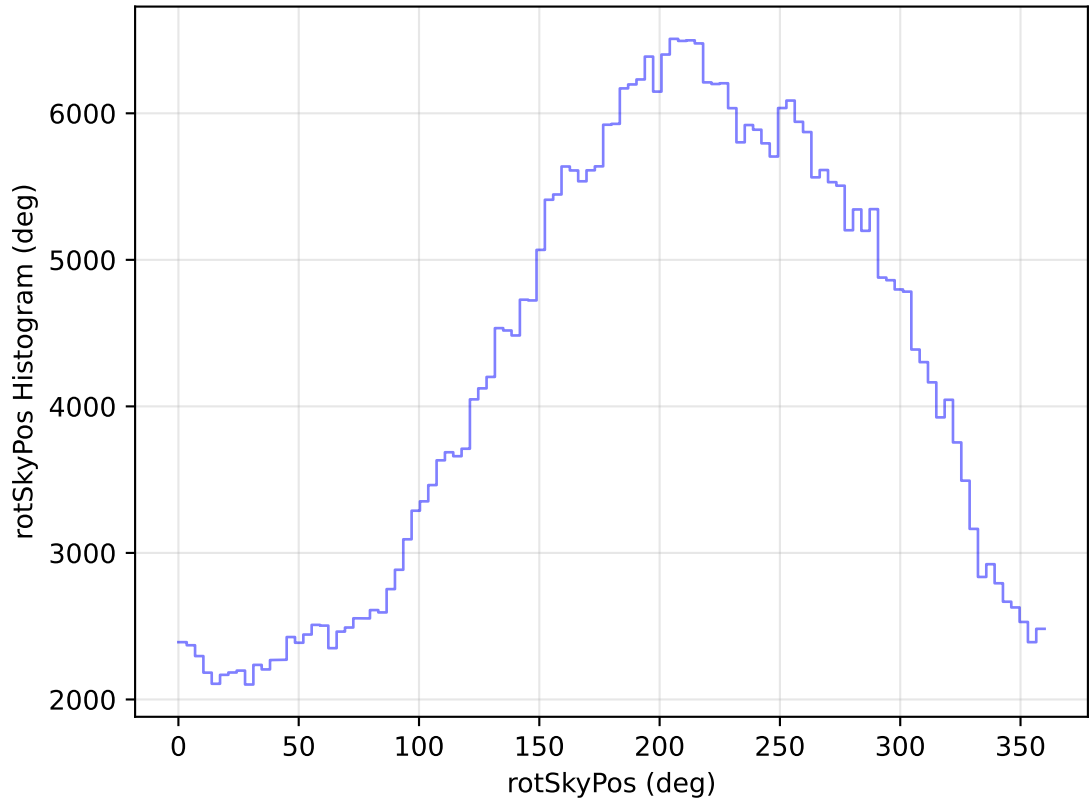
too_elab_heavy_r64_d2_ugrizy_v3.4_10yrs WFD z band: rotSkyPos Histogram
