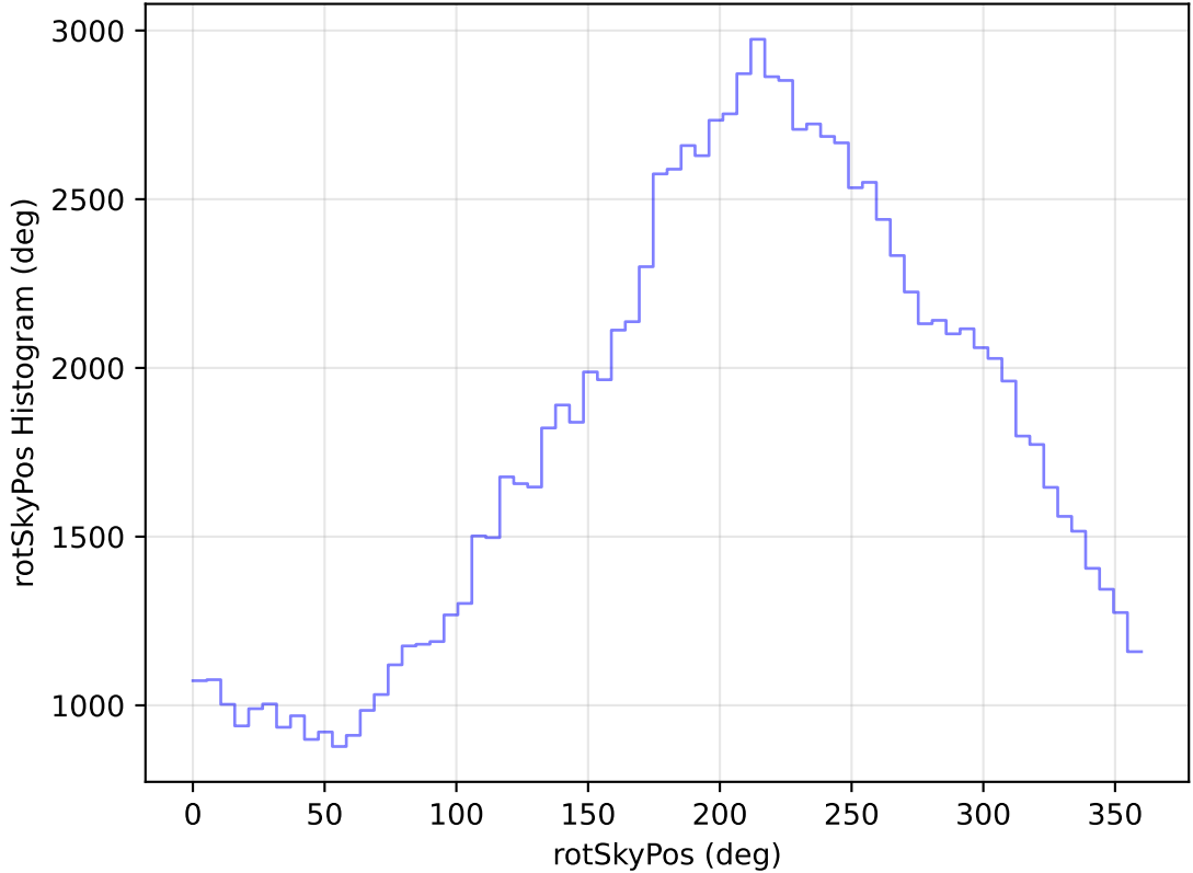
too_elab_heavy_r64_d2_ugrizy_v3.4_10yrs WFD u band: rotSkyPos Histogram
