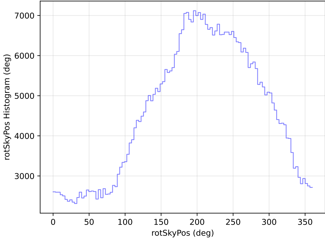
too_elab_heavy_r64_d2_ugrizy_v3.4_10yrs WFD i band: rotSkyPos Histogram
