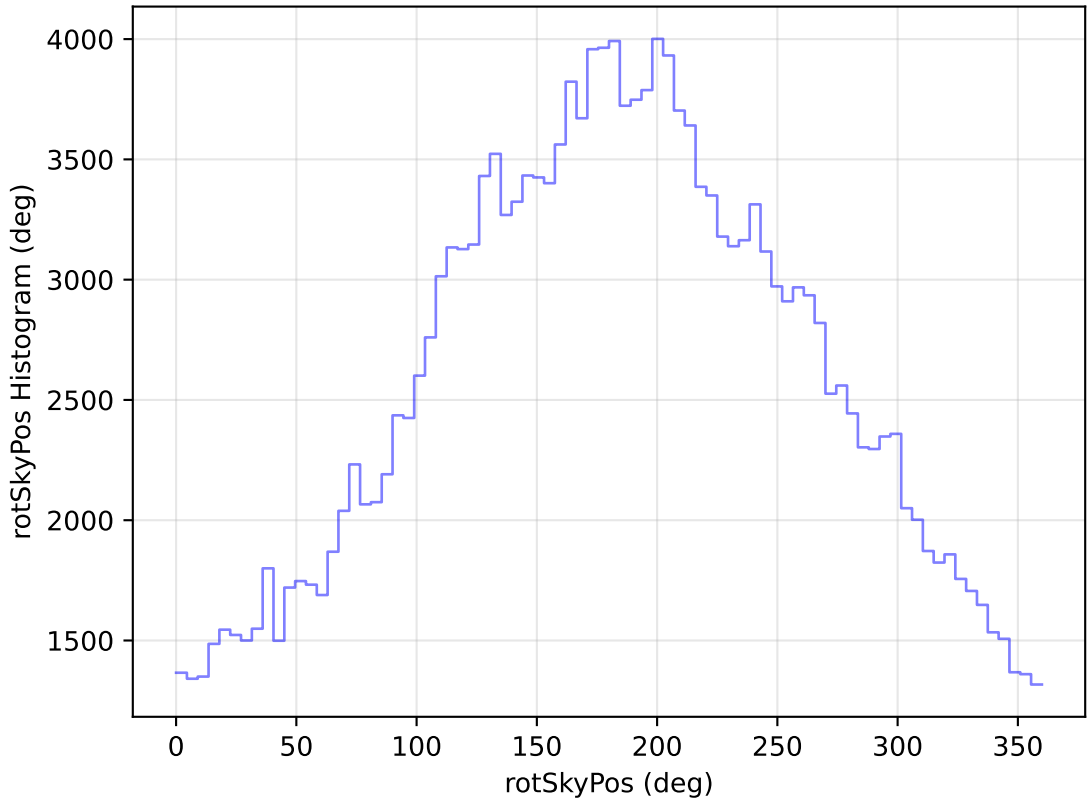
too_elab_heavy_r64_d2_ugrizy_v3.4_10yrs WFD g band: rotSkyPos Histogram
