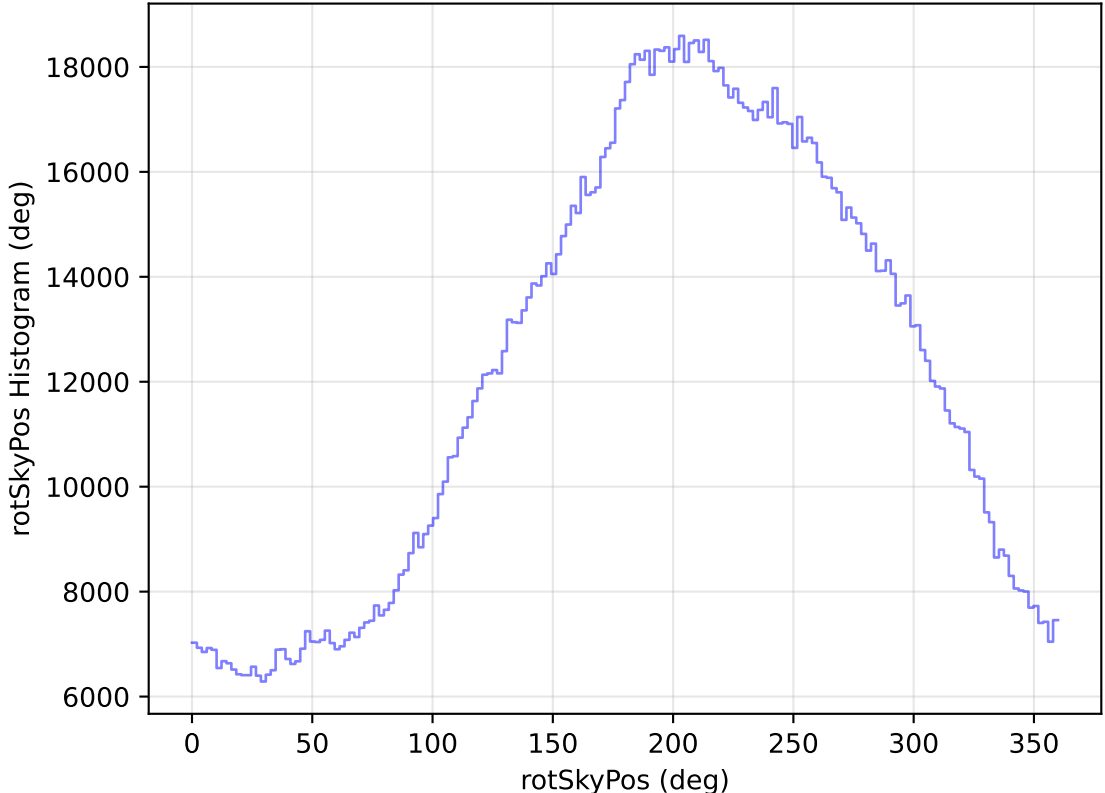
too_elab_heavy_r64_d2_ugrizy_v3.4_10yrs WFD all bands: rotSkyPos Histogram
