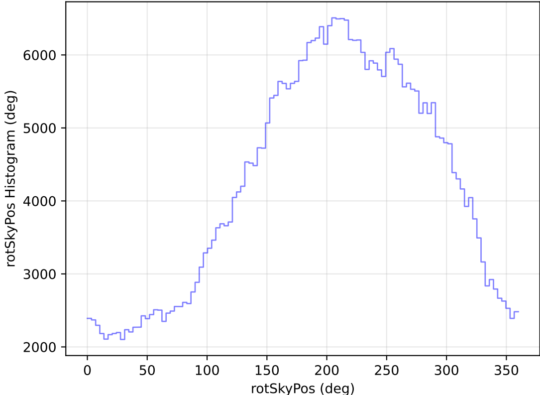
too_elab_heavy_r64_d2_ugrizy_v3.4_10yrs All sky z band: rotSkyPos Histogram
