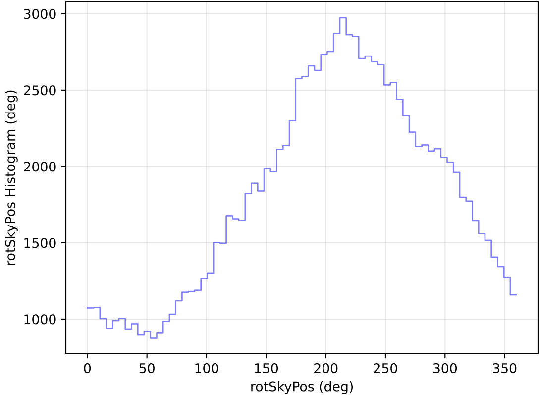
too_elab_heavy_r64_d2_ugrizy_v3.4_10yrs All sky u band: rotSkyPos Histogram
