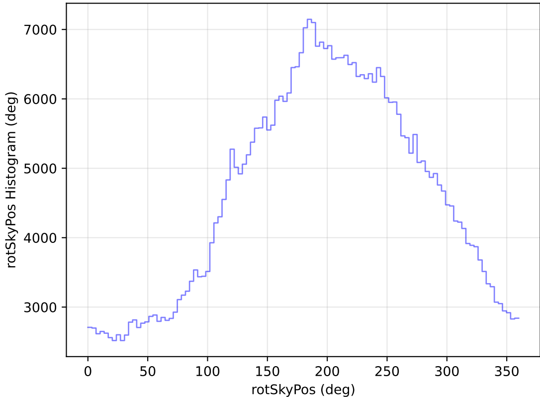
too_elab_heavy_r64_d2_ugrizy_v3.4_10yrs All sky r band: rotSkyPos Histogram
